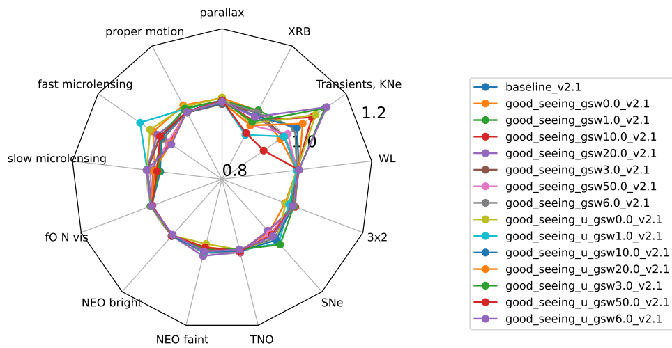
Figure 24. Observing some filters in good seeing conditions every year.
