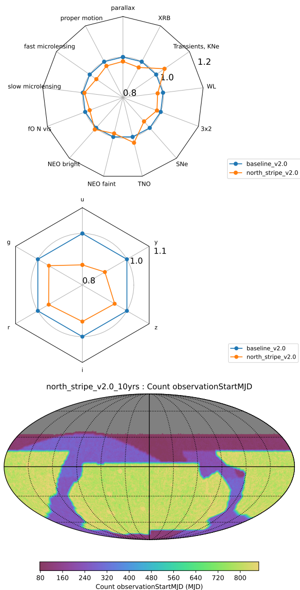
Figure 14. Impact of adding a northern stripe to the footprint.
