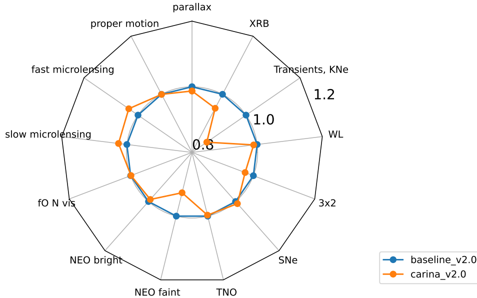
Figure 15. Impact of including the Carina microsurvey.
