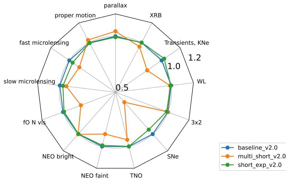
Figure 18. Impact of observing short exposure times.
