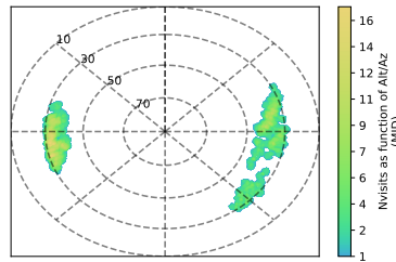
Figure 21. Number of visits in Alt,Az projection for the twilight NEO microsurvey. The top panel shows the standard 30s visit observations, middle panel shows 1s observations taken in twilight, and the bottom panel shows the twilight observations for one night.
