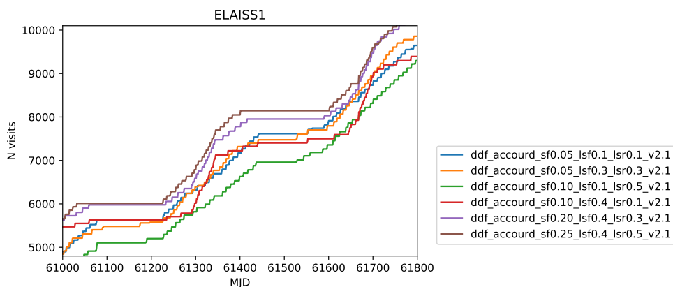
Figure 27. Examples of different DDF observing strategies. The season length, low cadence fraction, and low cadence rate are all varied.
