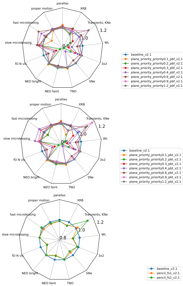
Figure 23. Looking at simulations with different galactic plane coverage. Top panel shows different footprints, middle panel shows the same footprints plus pencil beam surveys, and the bottom shows only pencil beam surveys.
