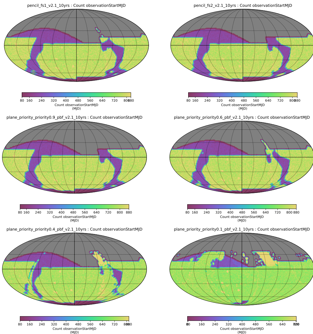
Figure 22. The various galactic plane footprints simulated.
