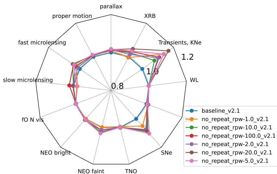
Figure 26. Suppressing repeat visits within a night. A boost for SNe, and an unexpected boost for the KNe metric.
