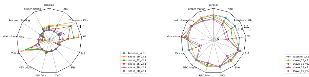
Figure 25. Trying different standard exposure times.
