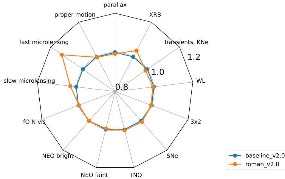
Figure 17. Impact of observing the Roman field.
