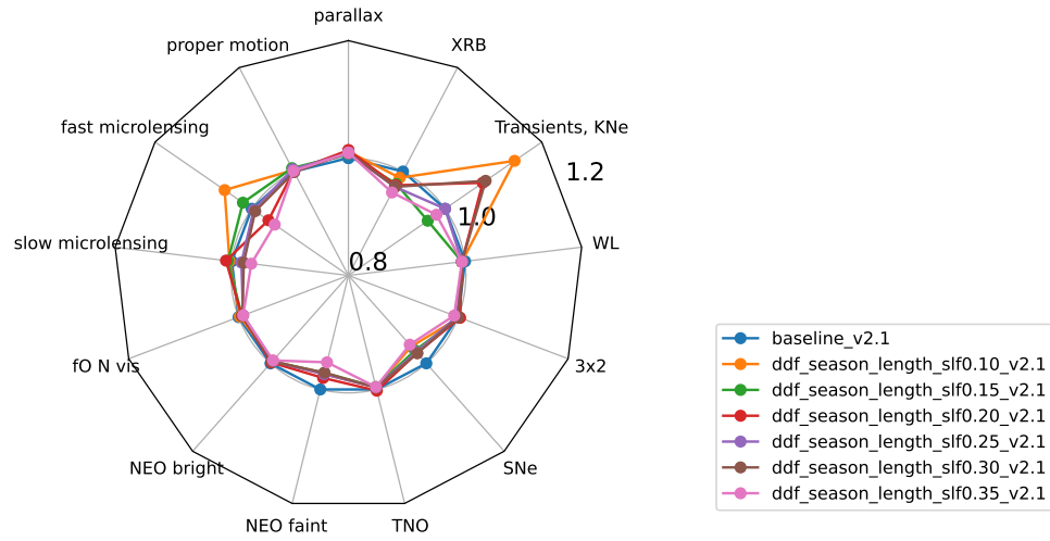
Figure 28. Shifting from the baseline to pre-scheduled DDF observations.
